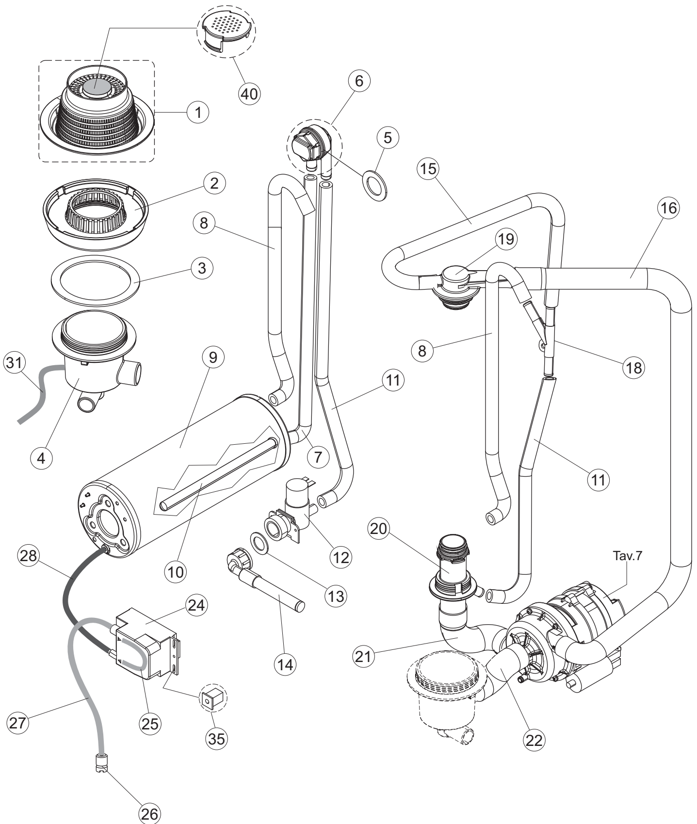
Drain Pump
